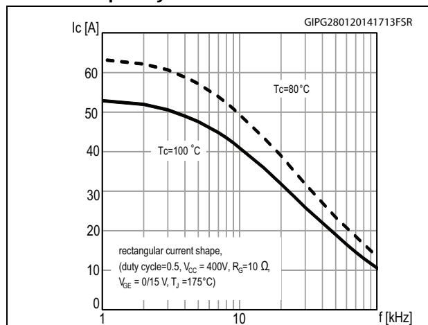
Figure 12. Collector current vs. switching frequency for TO-247 and TO-3P
