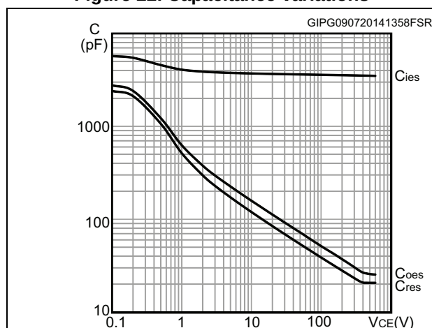
Figure 22. Capacitance variations
