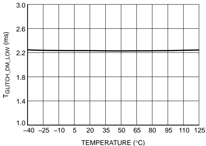
Figure 15. D- Low Glitch Filter, T GLITCH_DM_LOW
