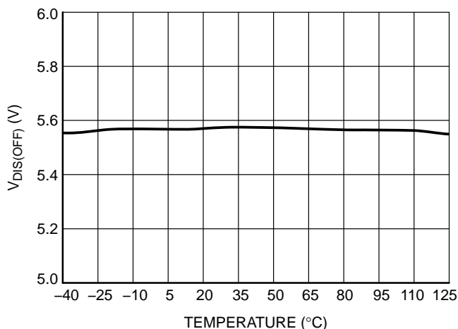
Figure 18. Discharge Comparator OFF Voltage, V DIS(OFF)
