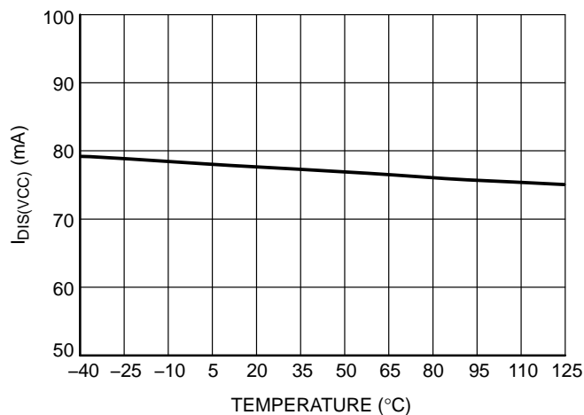
Figure 19. VCC Discharge Current, I DIS(VCC)
