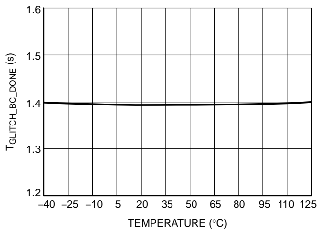
Figure 14. D+ High Glitch Filter Time, T_{GLITCH\_BC\_DONE}
