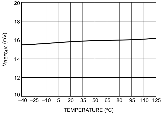
Figure 9. Current Control Reference Voltage, V_{REFC(A)}
