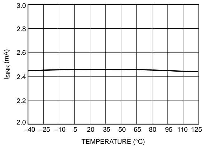
Figure 8. Voltage Control OTA Sink Current Capability, I_{SINKV}
