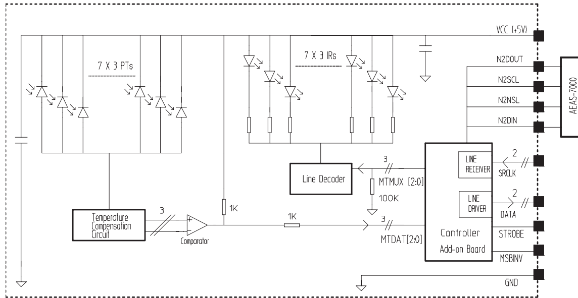
Figure 3. Block Diagram
