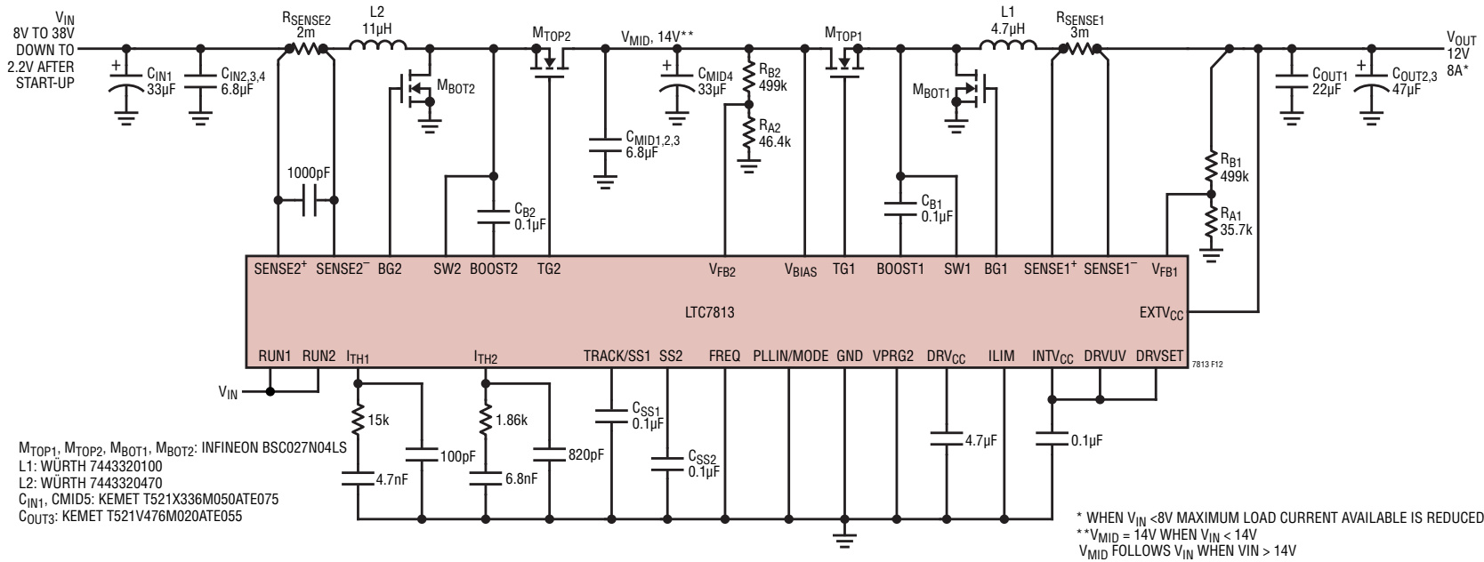
Figure 12. Wide Input Range to 12V/8A Low I_Q Cascaded Boost+Buck Regulator ( V_{MID} = 14V )
