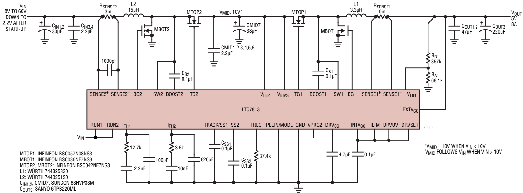
Figure 13. Wide Input Range to 5V/8A Low I Q Cascaded Boost+Buck Regulator (V MID Boosted to 10V)
