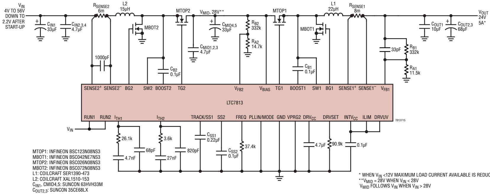
Figure 15. Wide Input Range to 24V/5A Low I q Cascaded Boost + Buck Regulator (V MID = 28V)
