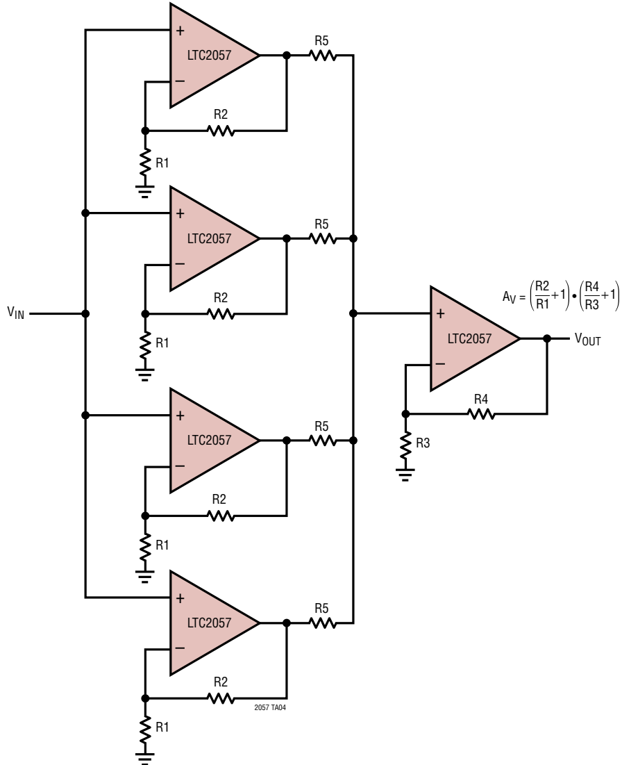
Paralleling Choppers to Improve Noise
