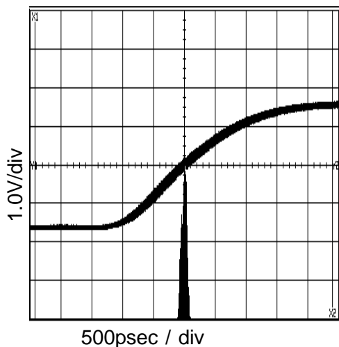
Figure 17. 18.4MHz Period-Jitter (V DD =3.3V, at C L =15pF)
