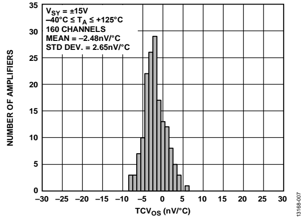
Figure 10. Input Offset Voltage Drift Distribution, V SY = ±15 V
