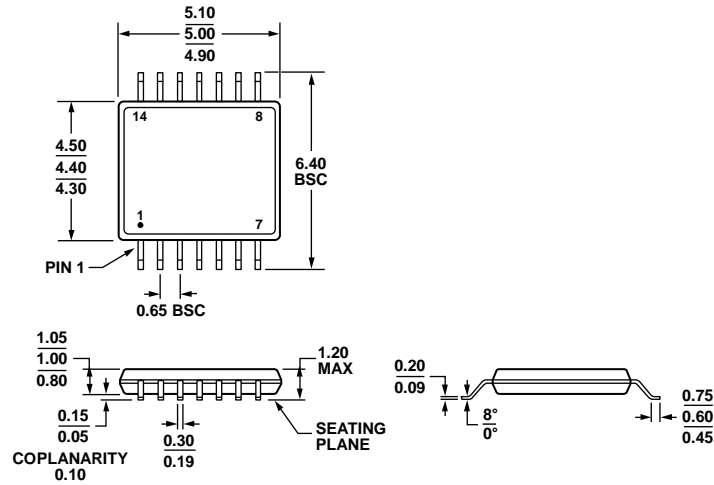
Figure 92. 14-Lead Thin Shrink Small Outline Package [TSSOP] (RU-14) Dimensions shown in millimeters
