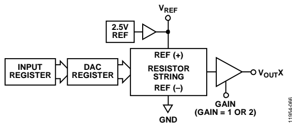
Figure 58. Single DAC Channel Architecture Block Diagram
