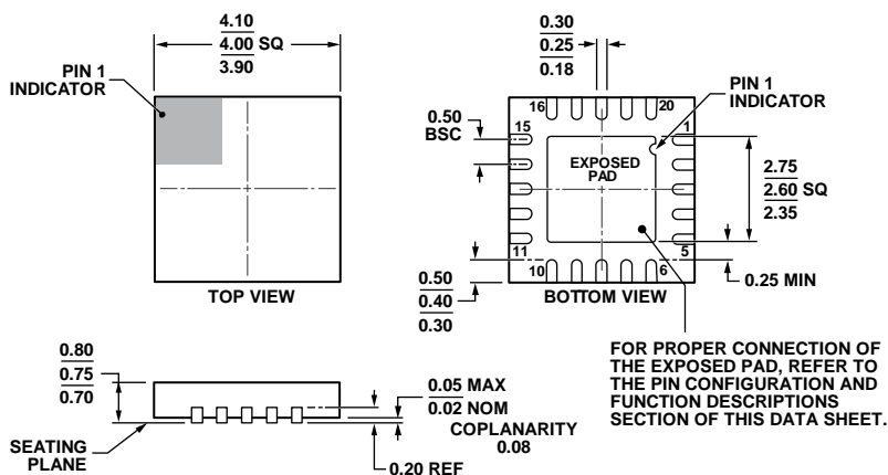
Figure 74. 20-Lead Lead Frame Chip Scale Package [LFCSP_WQ] 4 × 4 mm Body, Very Very Thin Quad (CP-20-8)
