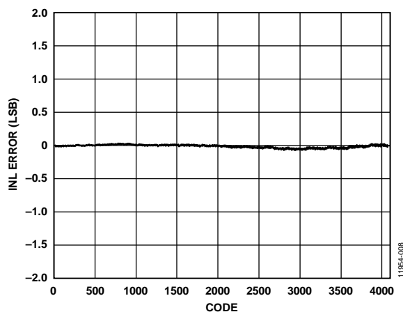
Figure 9. AD5672R INL Error vs. Code
