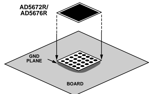
Figure 71. Pad Connection to the Board
