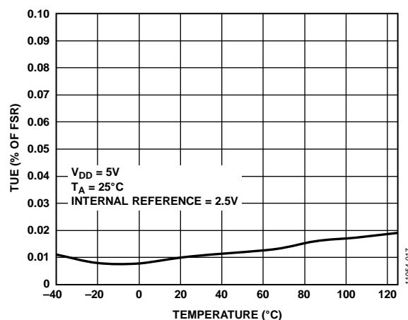
Figure 18. AD5676R TUE vs. Temperature
