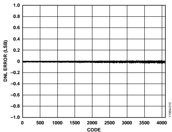
Figure 11. AD5672R DNL Error vs. Code
