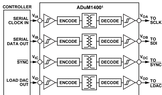
Figure 72. Isolated Interface
