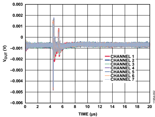
Figure 45. Analog Crosstalk
