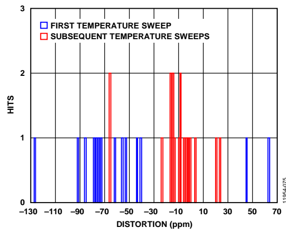
Figure 67. Thermal Hysteresis
