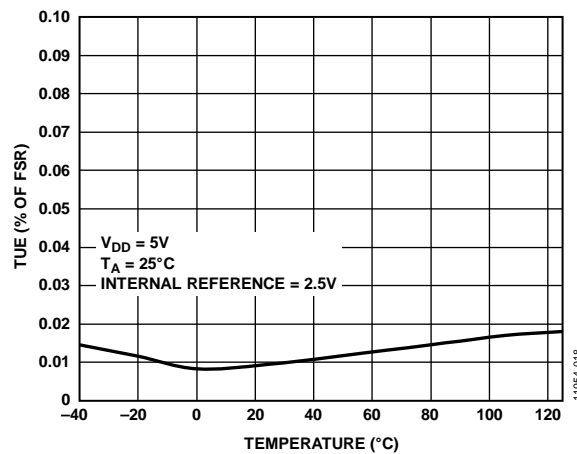
Figure 19. AD5672R TUE vs. Temperature
