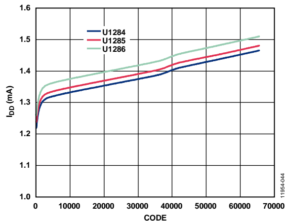
Figure 37. Supply Current ( I_{DD} ) vs. Code
