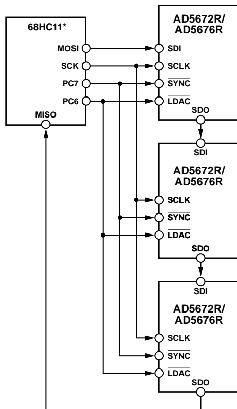
Figure 62. Daisy-Chaining the AD5672R/AD5676R
