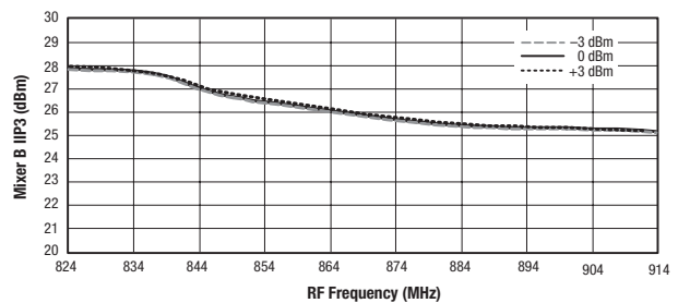
Figure 18. Mixer B IIP3 vs Frequency and LO Power
