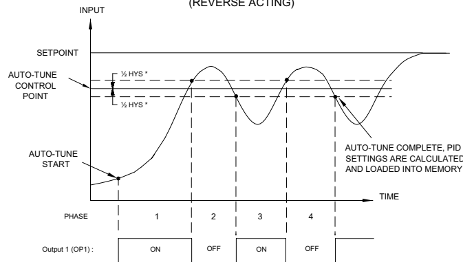
AUTO-TUNE OPERATION (REVERSE ACTING)
