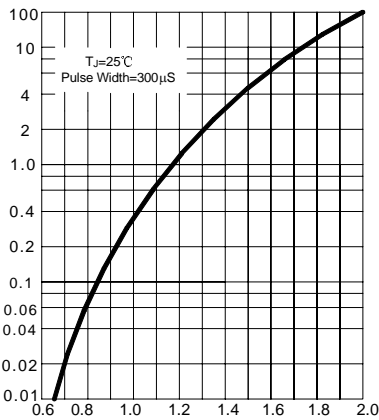
FIG.2 – TYPICAL FORWARD CHARACTERISTIC
