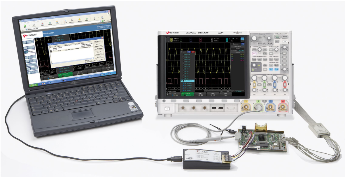
Figure 1. FPGA dynamic probe for Xilinx used in conjunction with a Keysight InfiniiVision 6000, 7000, or 4000 or 6000 X-Series MSO provides an effective solution for simple through complex debugging of systems incorporating Xilinx FPGAs.
