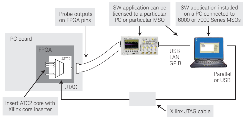
Figure 2. Create a timesaving FPGA measurement system. Insert an ATC2 (Keysight Trace Core) core into your FPGA design. With the application running on your PC you control which group of internal signals to measure via JTAG.
