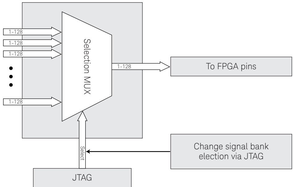
Figure 3. Access up to 64 internal signals for each debug pin. Signal banks all have identical width (1 to 128 signals wide) determined by the number of device pins you devote for debug. Each pin provides sequential access to one signal from every input bank.
