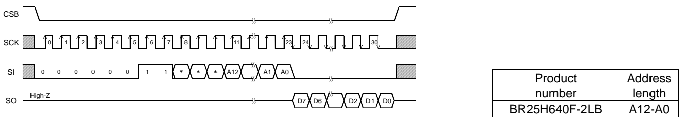
Figure 37. Read command
