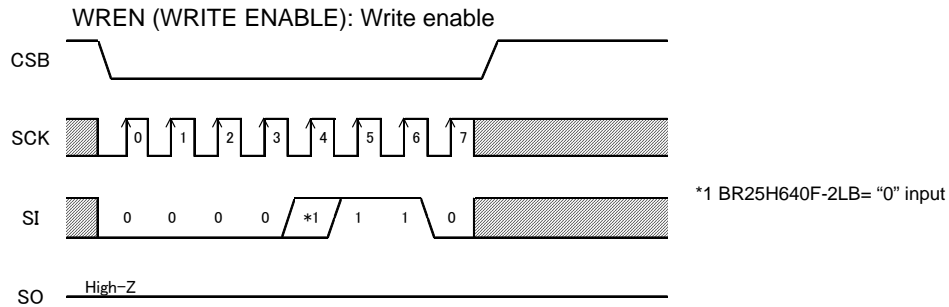
Figure 35. Write enable command
