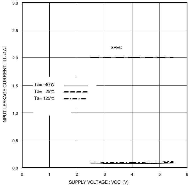
Figure 11. Input Leakage Current IILI (CSB,SCK,SI,HOLDB,WPB)
