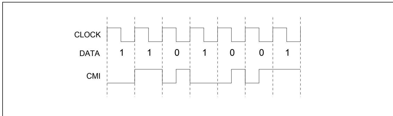
Figure 24-2. CMI Coding
