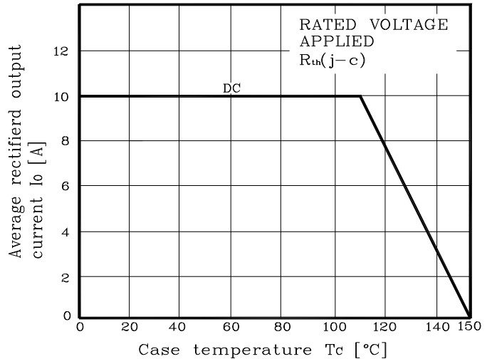
Fig. 6 I_O \text{ derating} - T_C
