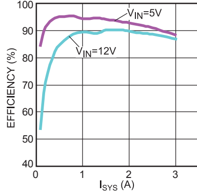
Efficiency vs. System Current
