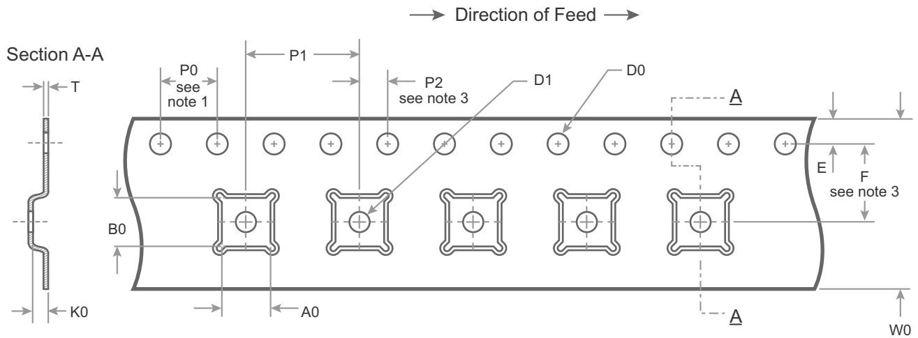
Figure 23 • Tape and Reel Specifications for 32-lead 5 × 5 × 0.85 mm QFN
