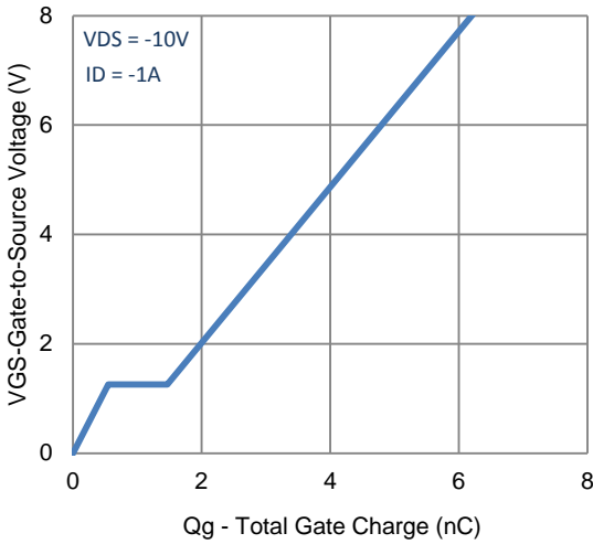
7. Gate Charge
