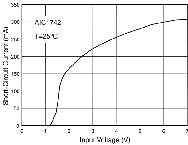
Fig. 3 Short-Circuit Current
