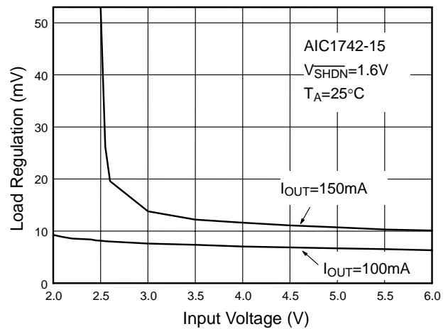
Fig. 6 Load Regulation
