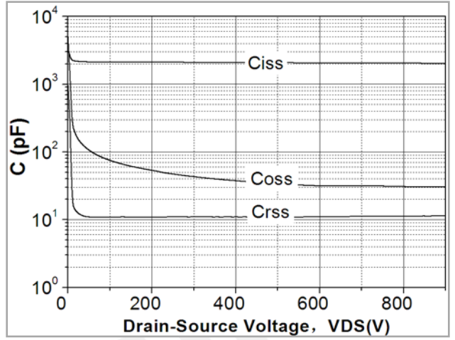
Fig. 8. Capacitance Characteristics
