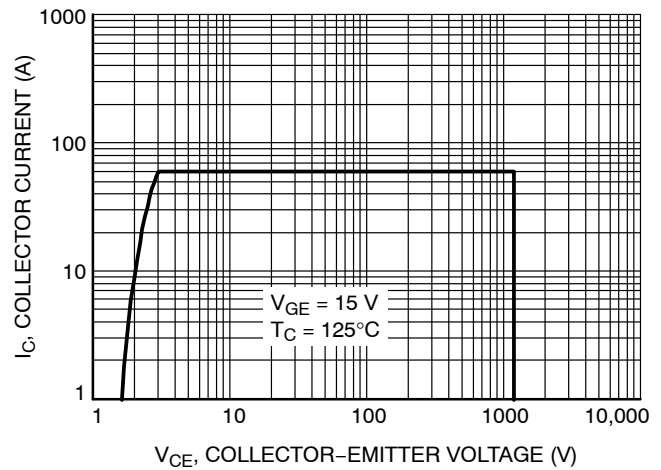
Figure 18. I_C vs. V_{CE}
