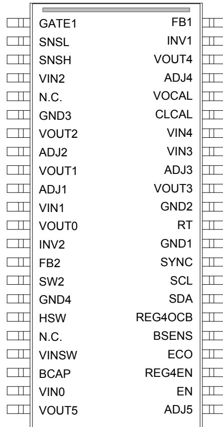
Figure 1. Pin Configuration(s)
