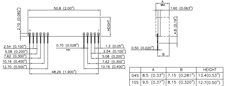
BACK VIEW
