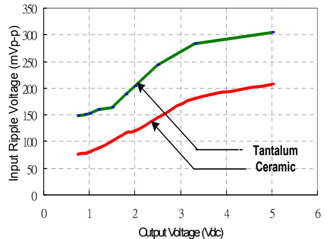
Figure 20: Input ripple voltage for various output models, I_o = 16A ( C_{in} = 6 \times 47\mu F tantalum capacitors and 6 \times 22\mu F ceramic capacitors at the input)
