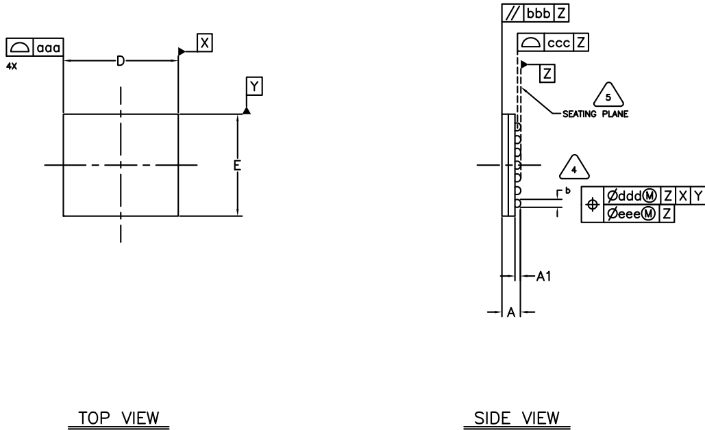
Figure 18. CYW20710A1KUFBXG Mechanical Drawing
