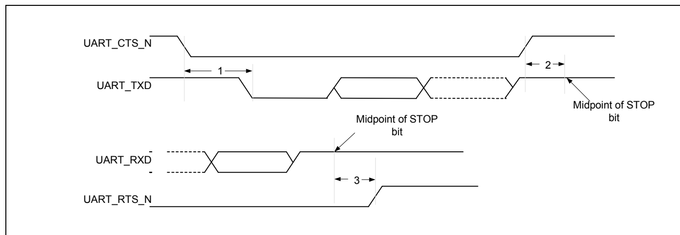
Figure 12. UART Timing
