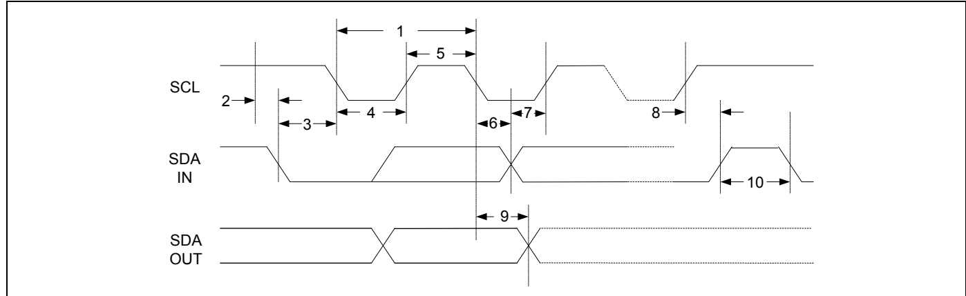
Figure 17. BSC Interface Timing Diagram
