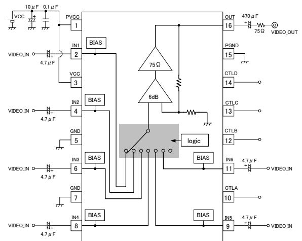
Fig.8 BH76361FV
