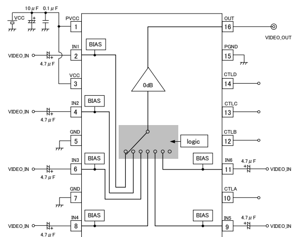
Fig.10 BH76363FV
