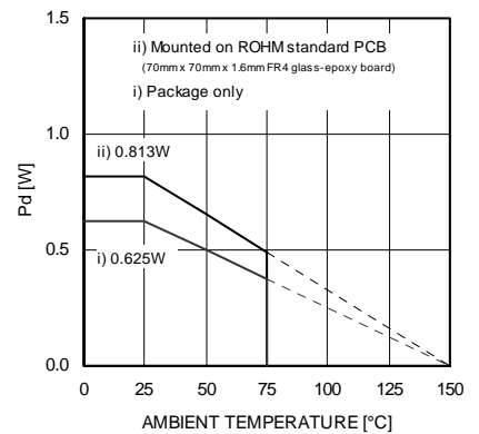
Fig.12 Thermal derating curve (SSOP-A16)
