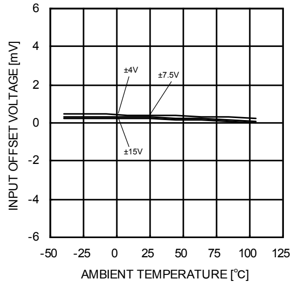
Figure 55. Input Offset Voltage - Ambient Temperature ( V_{ICM}=0V , V_{OUT}=0V )
