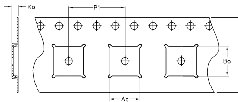
TAPE DIMENSIONS
