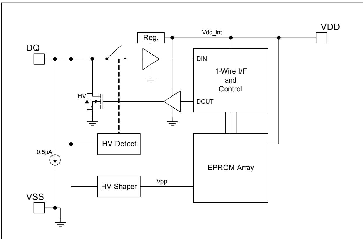
Figure 1. Block Diagram
