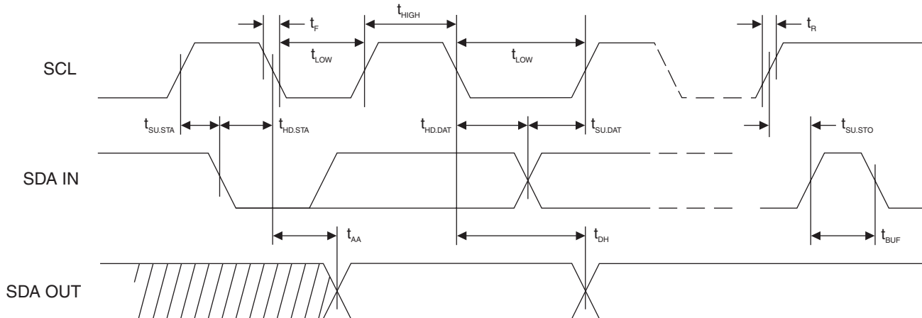
Figure 3-2. Write Cycle Timing SCL: Serial Clock, SDA: Serial Data I/O
