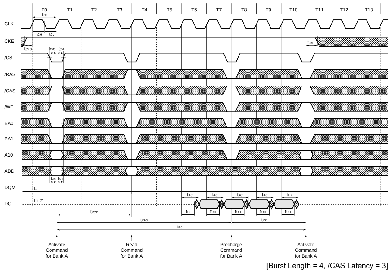
AC Parameters for Read Timing with Manual Precharge
