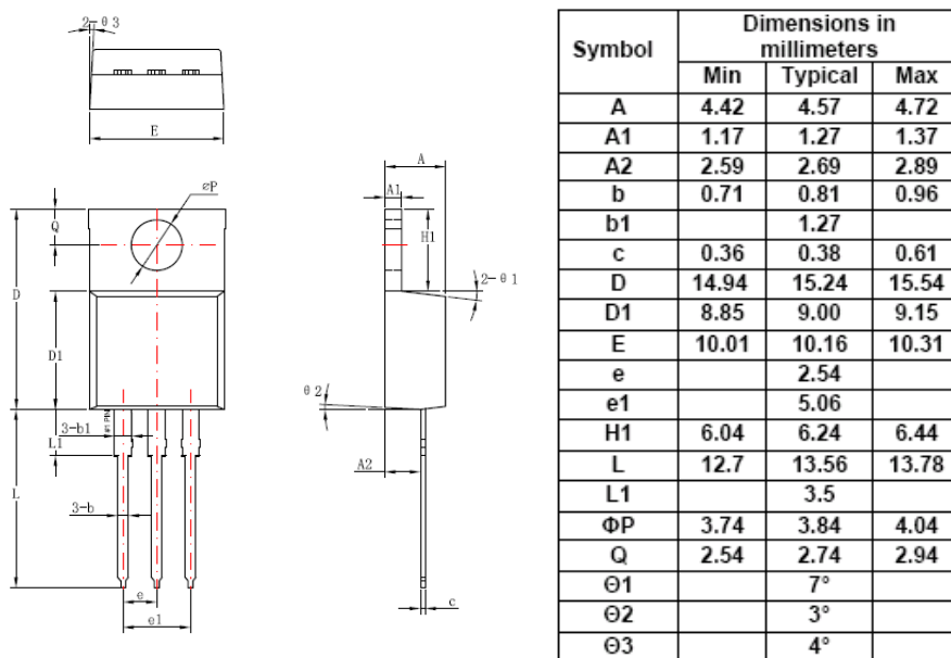
Mechanical Dimensions: In Inches / mm
