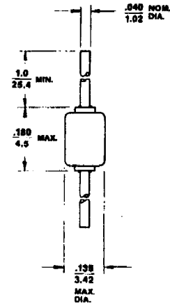
FIGURE 1 PACKAGE E
