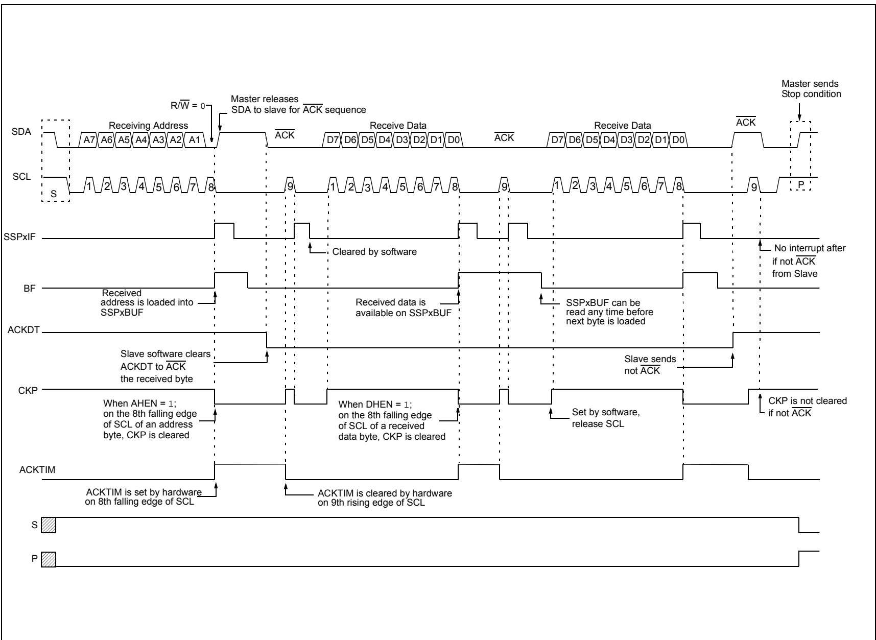
FIGURE 29-17: I 2 C SLAVE, 7-BIT ADDRESS, RECEPTION (SEN = 1, AHEN = 1, DHEN = 1)
