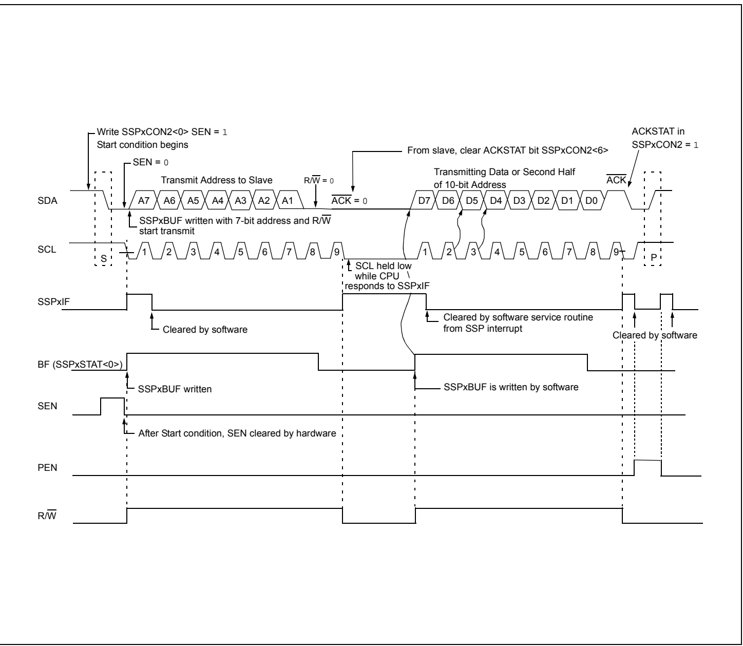
FIGURE 29-28: I 2 C MASTER MODE WAVEFORM (TRANSMISSION, 7 OR 10-BIT ADDRESS)
