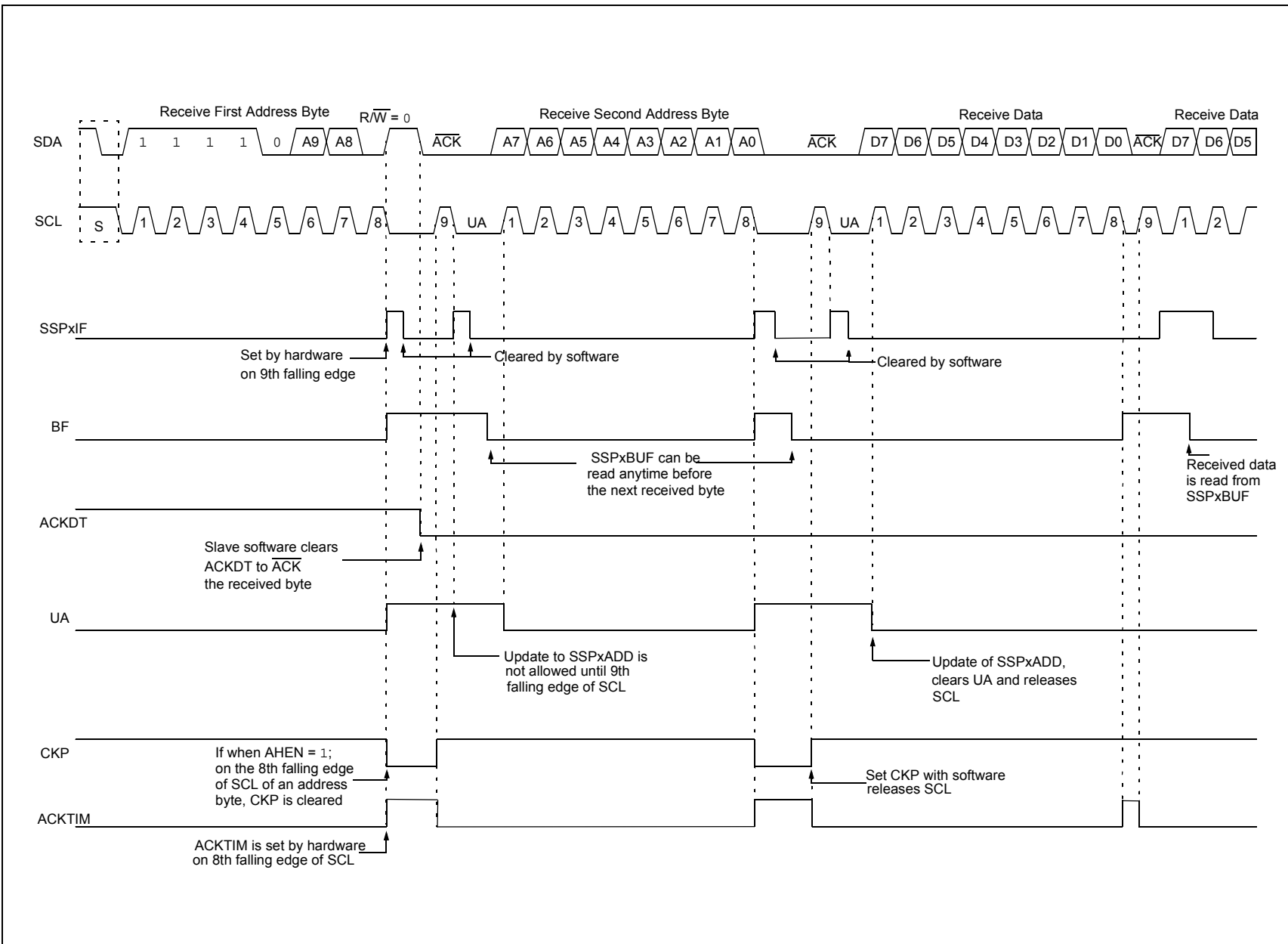
FIGURE 29-21: I 2 C SLAVE, 10-BIT ADDRESS, RECEPTION (SEN = 0, AHEN = 1, DHEN = 0)
