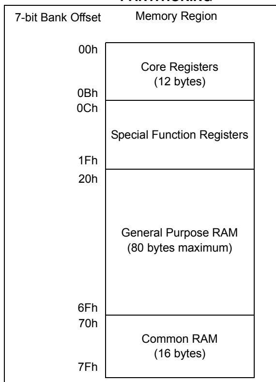
FIGURE 3-2: BANKED-MEMORY PARTITIONING
