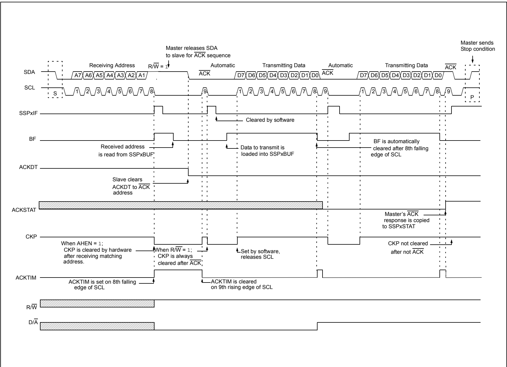
FIGURE 29-19: I 2 C SLAVE, 7-BIT ADDRESS, TRANSMISSION (AHEN = 1)
