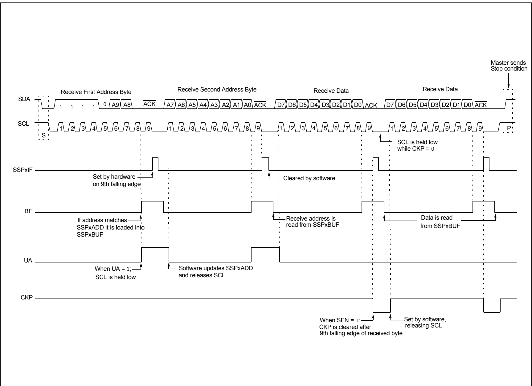
FIGURE 29-20: I 2 C SLAVE, 10-BIT ADDRESS, RECEPTION (SEN = 1, AHEN = 0, DHEN = 0)
