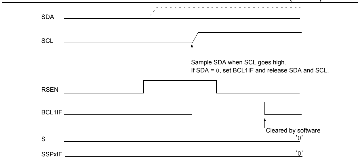
FIGURE 29-36: BUS COLLISION DURING A REPEATED START CONDITION (CASE 1)
