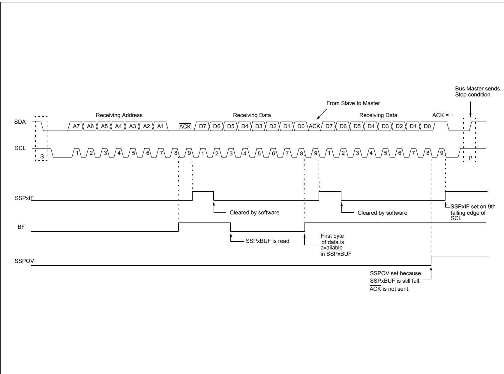
FIGURE 29-14: I 2 C SLAVE, 7-BIT ADDRESS, RECEPTION (SEN = 0, AHEN = 0, DHEN = 0)
