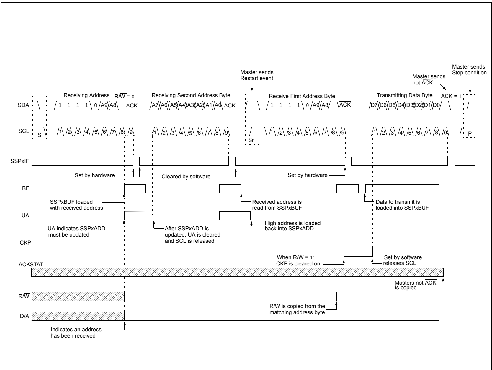
FIGURE 29-22: I 2 C SLAVE, 10-BIT ADDRESS, TRANSMISSION (SEN = 0, AHEN = 0, DHEN = 0)
