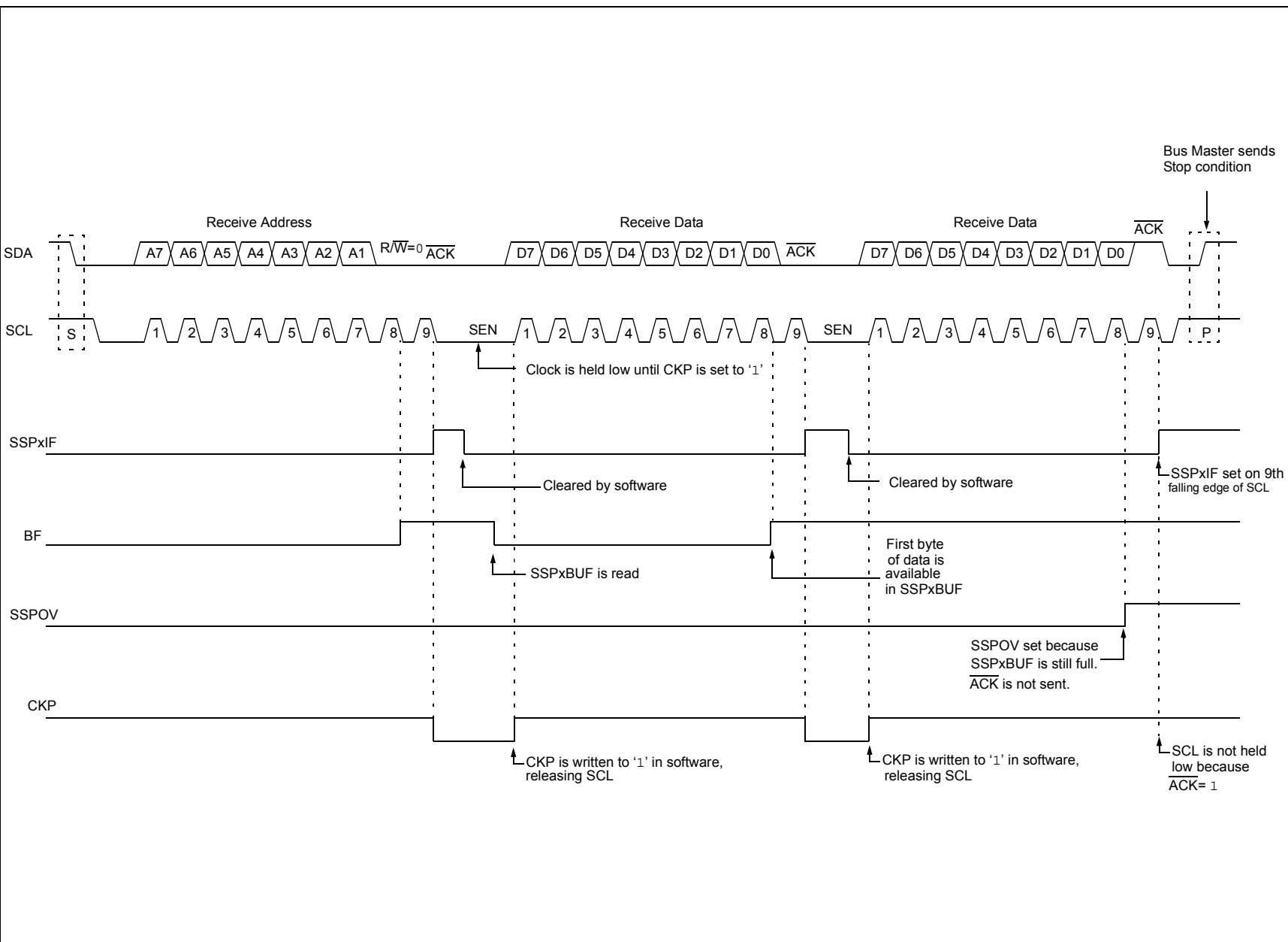
FIGURE 29-15: I 2 C SLAVE, 7-BIT ADDRESS, RECEPTION (SEN = 1, AHEN = 0, DHEN = 0)
