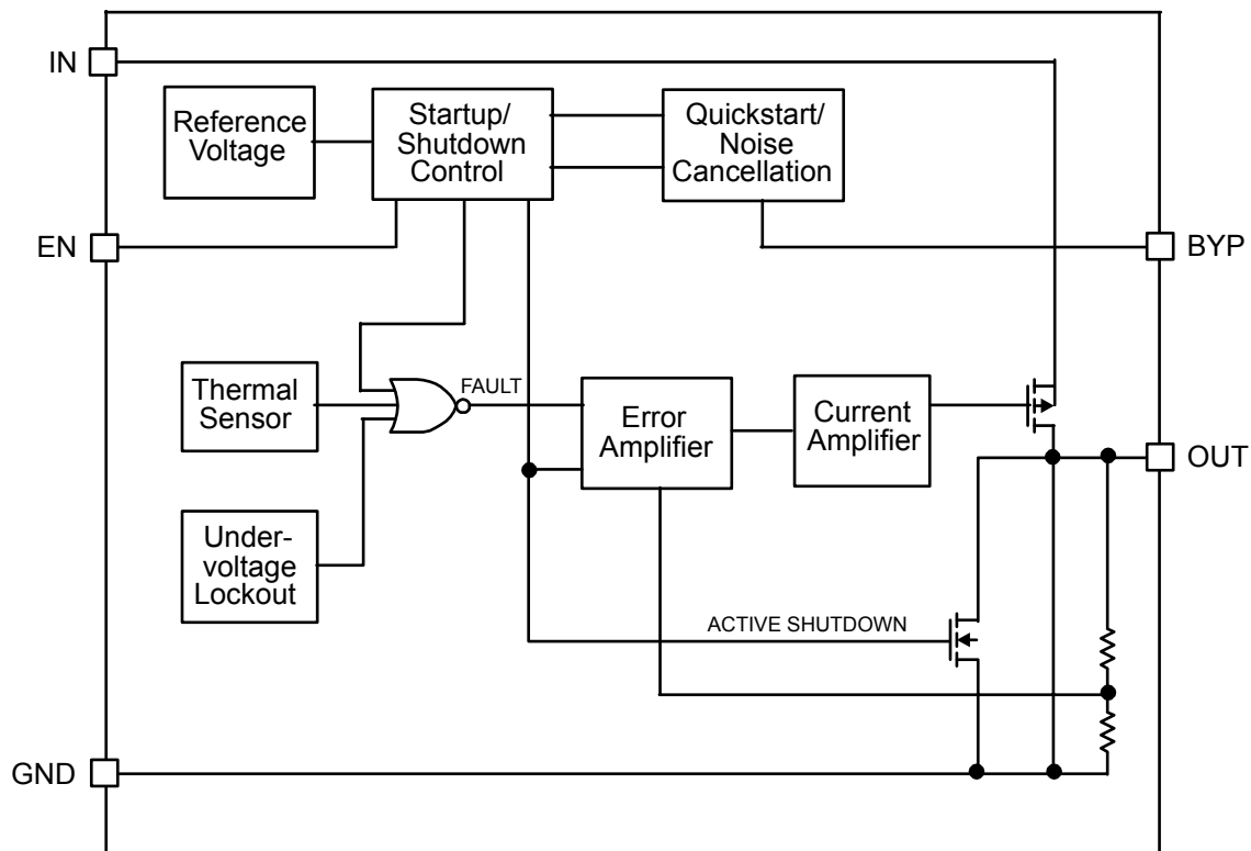
MIC5265 Diagram
