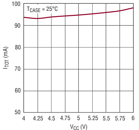
Total Current ( I_{TOT} ) vs V_{CC}
