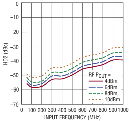
HD2 vs Frequency Over P_{OUT}
