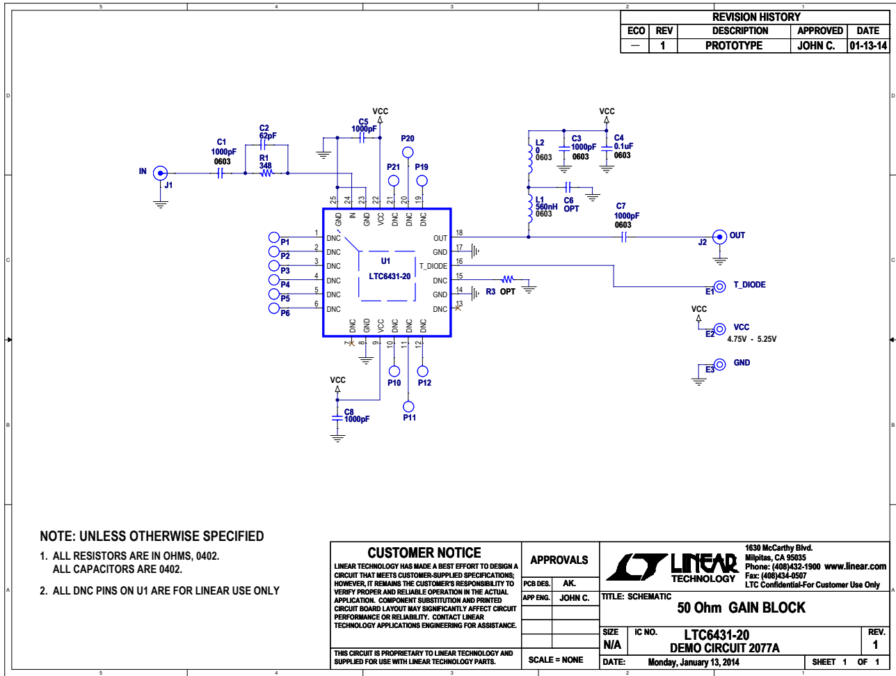
Figure 2. DC2077A Demo Board Schematic
