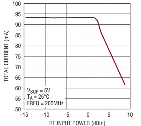
Total Current vs RF Input Power
