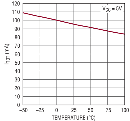
Total Current ( I_{TOT} ) vs Temperature
