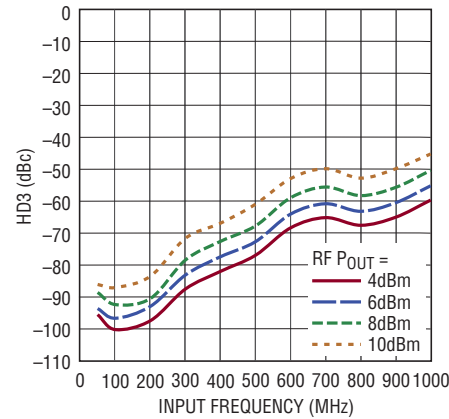
HD3 vs Input Frequency Over P_{OUT}
