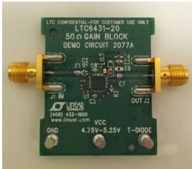
Figure 3. Demo Board
