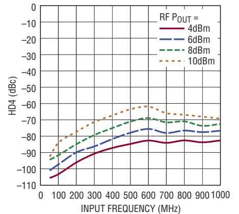
HD4 vs Input Frequency Over P_{OUT}
