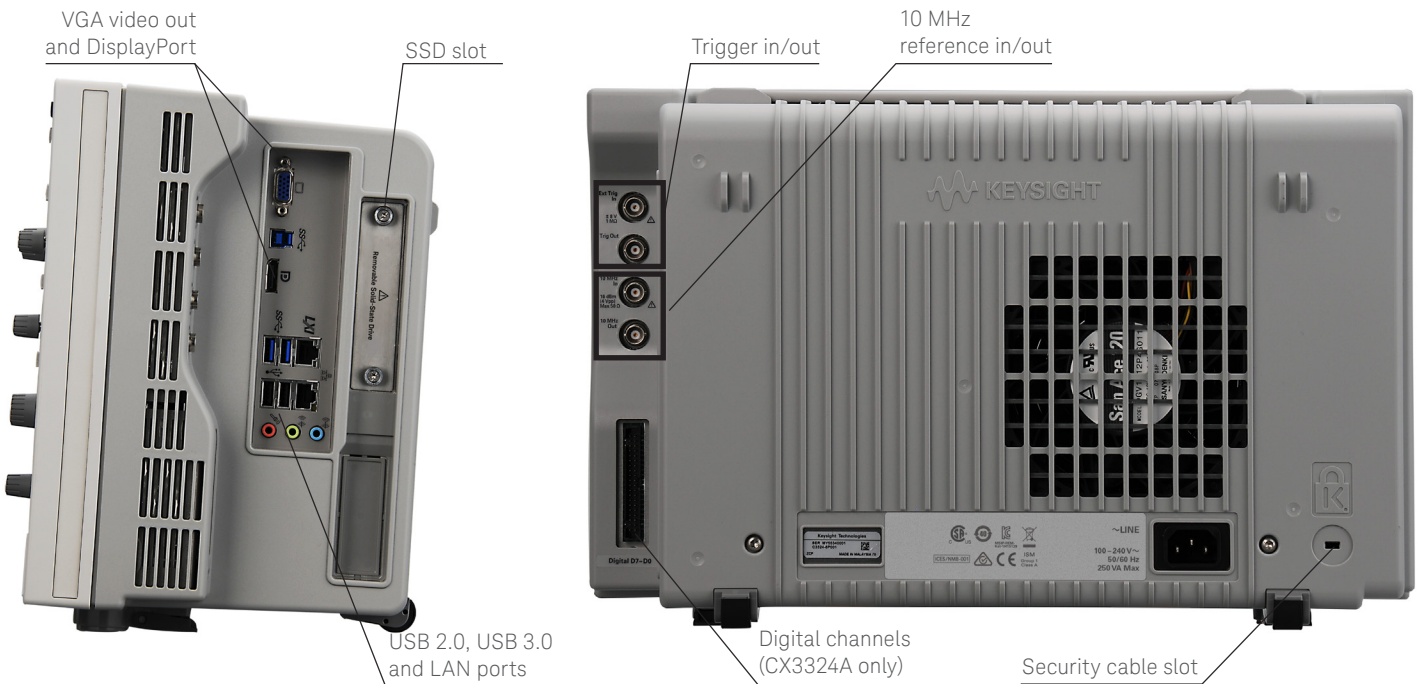
Figure 22. CX3324A front, rear and side views
