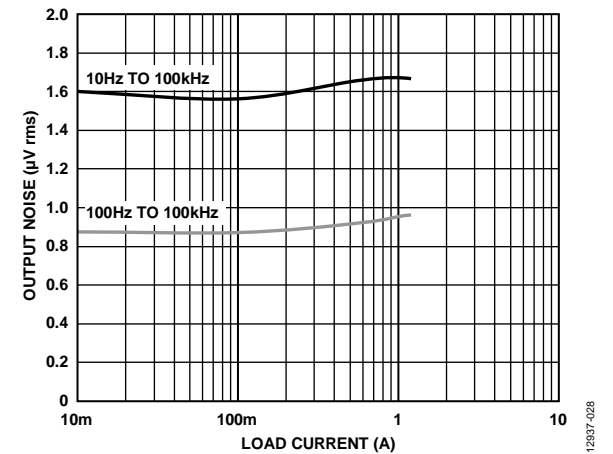
Figure 28. RMS Output Noise vs. Load Current
