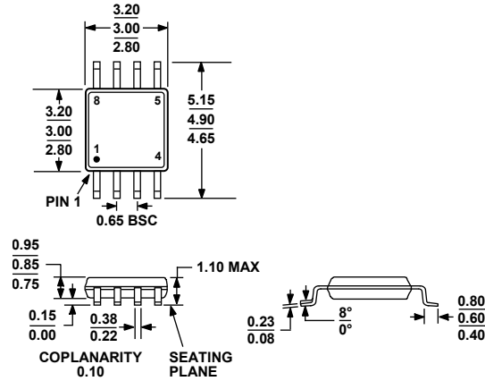
Figure 55. 8-Lead Mini Small Outline Package [MSOP]
