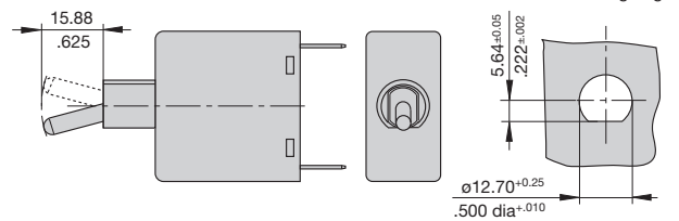
Baton actuator threadneck mounting
