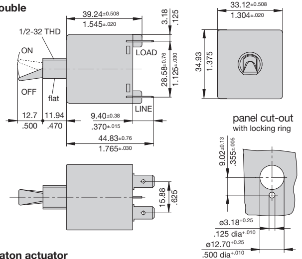
Baton actuator threadneck mounting
