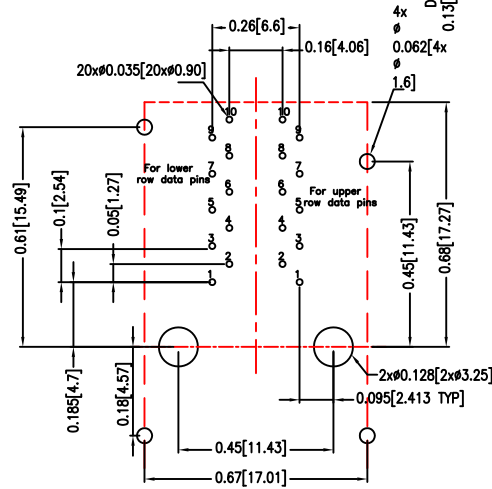
P.C.B RECOMMENDED HOLE LAYOUT SEEN FROM COMPONENT SIDE
