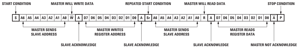
Figure 9. Register Byte Read Protocol.
