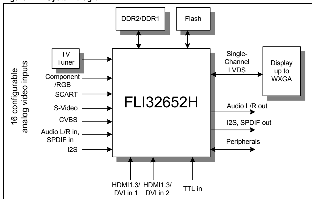
Figure 1. System diagram
