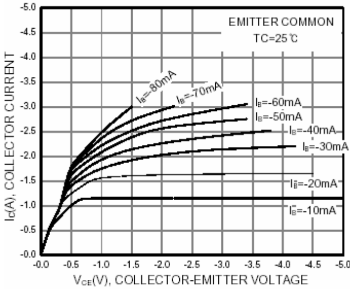
Fig.3 Static Characteristic
