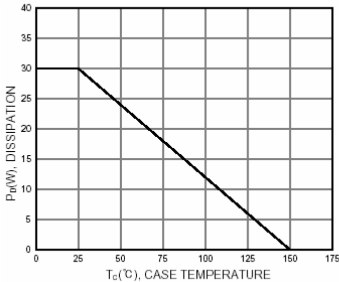
Fig.7 Power Derating
