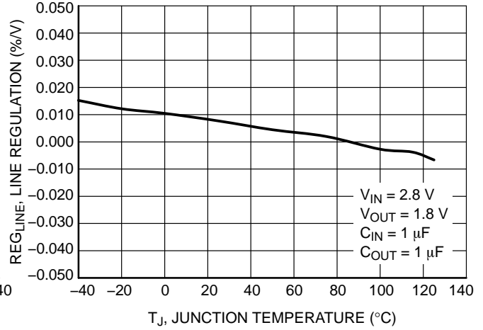
Figure 6. Line Regulation vs. Temperature – V OUT = 1.8 V
