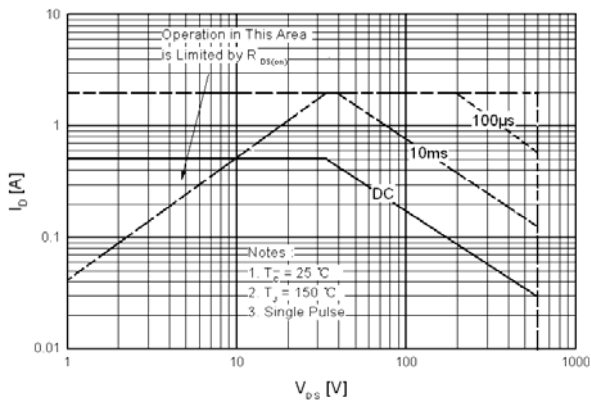
Maximum Safe Operating Area For JCS1HN65TC
