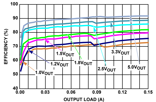
FIGURE 2. EFFICIENCY vs LOAD, PFM, V_{IN} = 12\text{V}
