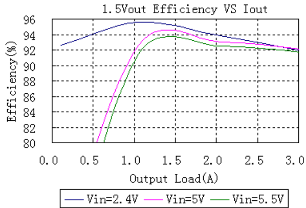
Figure 3: Converter efficiency vs. output current (1.5V out)
