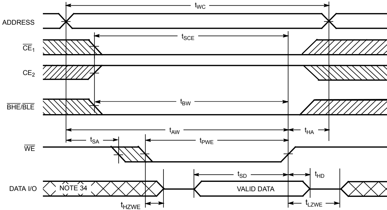
Figure 10. Write Cycle No. 3 ( \overline{WE} Controlled, \overline{OE} LOW) [33]
