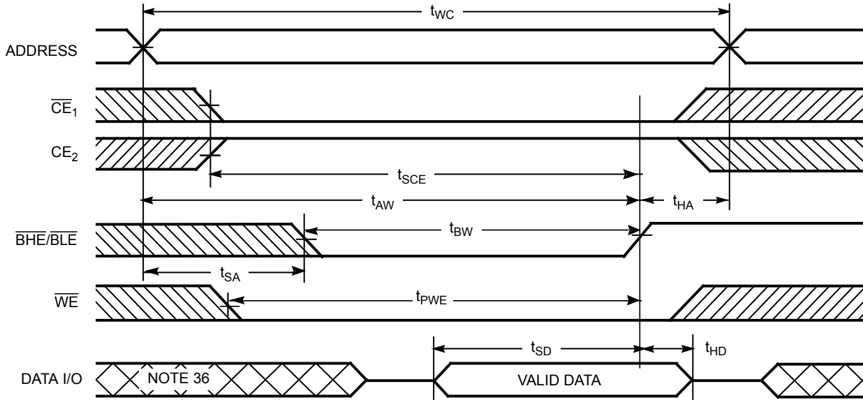
Figure 11. Write Cycle No. 4 ( \overline{\text{BHE}}/\overline{\text{BLE}} Controlled, \overline{\text{OE}} LOW) [35]
