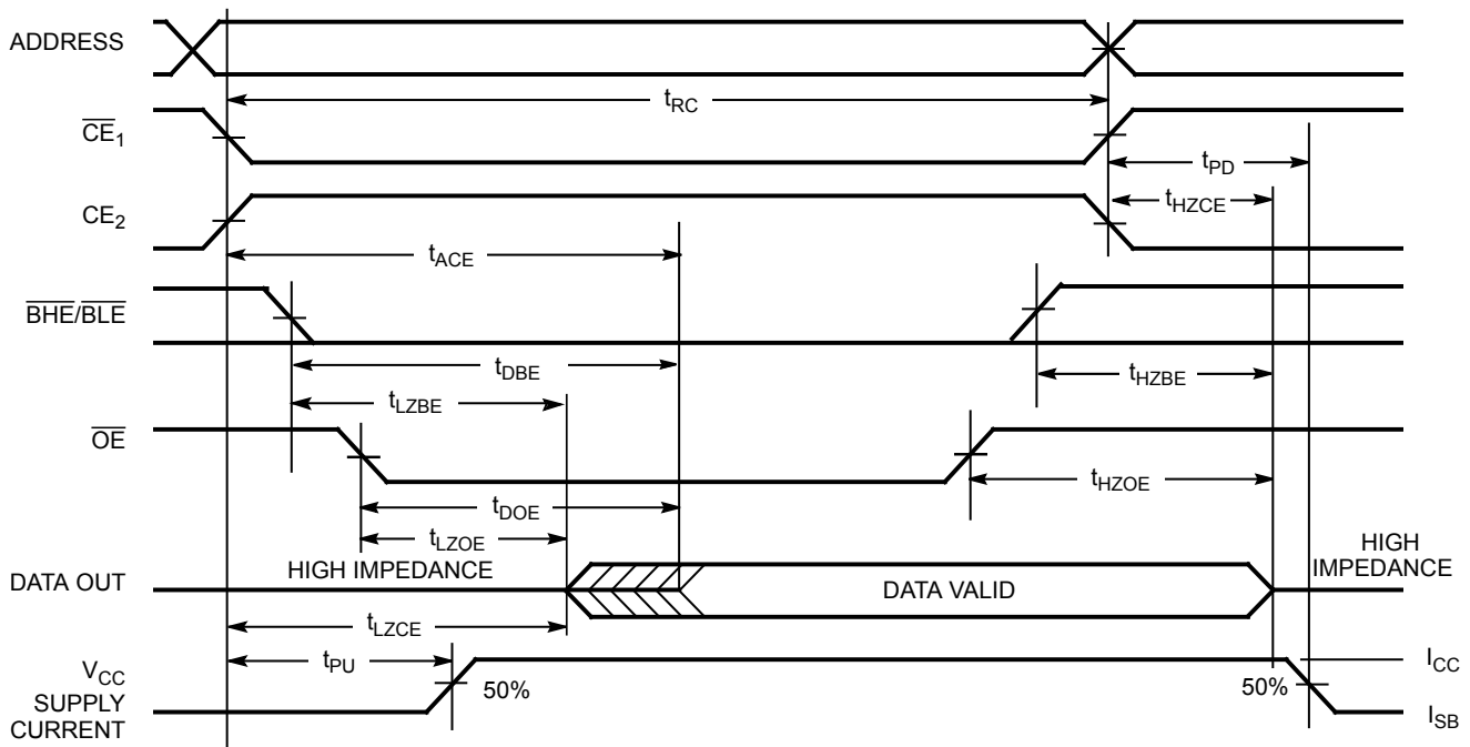
Figure 7. Read Cycle No. 2 ( \overline{OE} Controlled) [23, 24]
