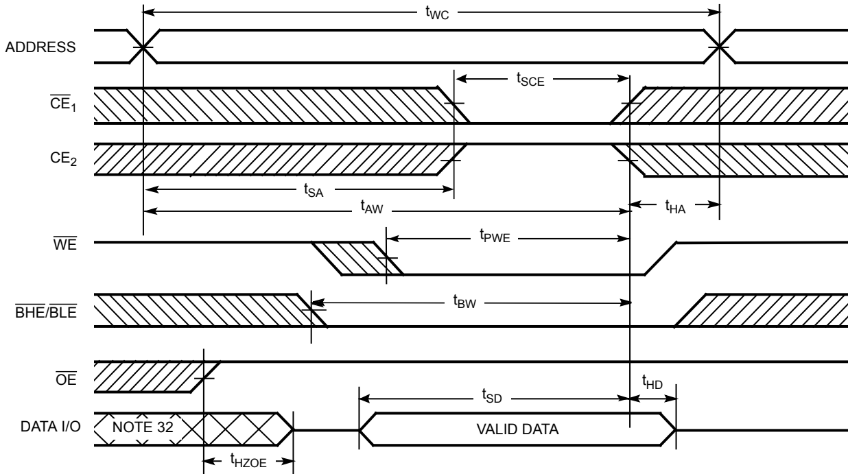
Figure 9. Write Cycle No. 2 ( \overline{CE}_1 or CE_2 Controlled) [29, 30, 31]
