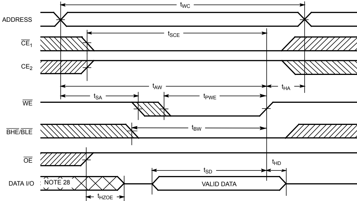
Figure 8. Write Cycle No. 1 ( \overline{WE} Controlled) [25, 26, 27]
