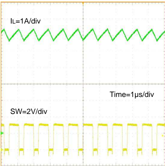
Figure 34. Switching Waveform (VIN= 3.3V, VOUT= 1.8V, IOUT= 6A, L= 1.0μH)
