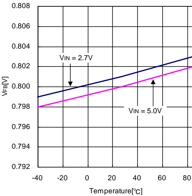
Figure 7. FB Voltage Reference vs Temperature
