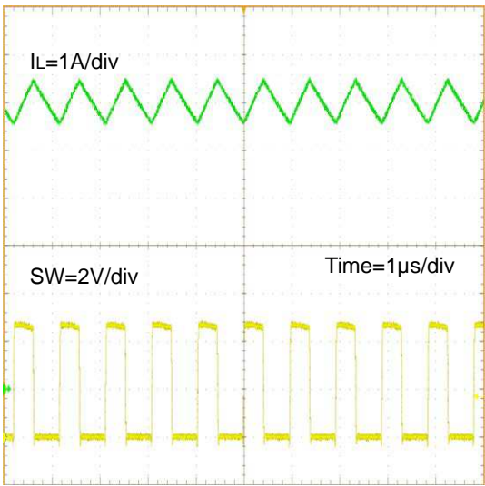
Figure 35. Switching Waveform (VIN= 5.0V, VOUT= 1.8V, IOUT= 6A, L= 1.5μH)
